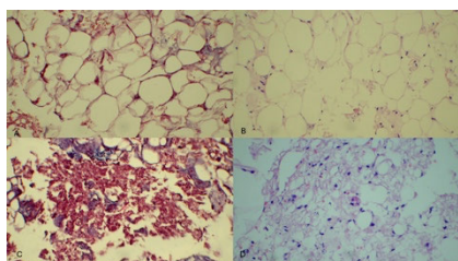
Figure 1:DPAT analysis
